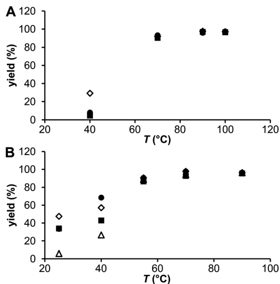
Fig. 6 Radiolabeling of DOTA (●) and its monophasphorus acid analogues (◇ DO3AP, ■ DO3AP ABn and △ DO3AP PrA ) at different temperatures (pH 4.0, labelling time 30 min): (A) generator 44 Sc, n(\text{ligand}) = 20 \text{ nmol} ; n(\text{Sc}) = 4.5 \times 10^{-5} to 1 \times 10^{-4} \text{ nmol} ; A(^{44}\text{Sc}) = 3 \text{ kBq} . (B) Cyclotron 44m Sc/ 44 Sc, n(\text{ligand}) = 0.2 \text{ nmol} ; n(\text{Sc}) = 1.5 \times 10^{-6} \text{ nmol} ; A(^{44}\text{Sc}) = 3 \text{ kBq} .
